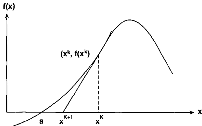
Figure 8. Newton-Raphson method.
