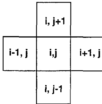
Figure 10. Computational molecule (or stencil).
