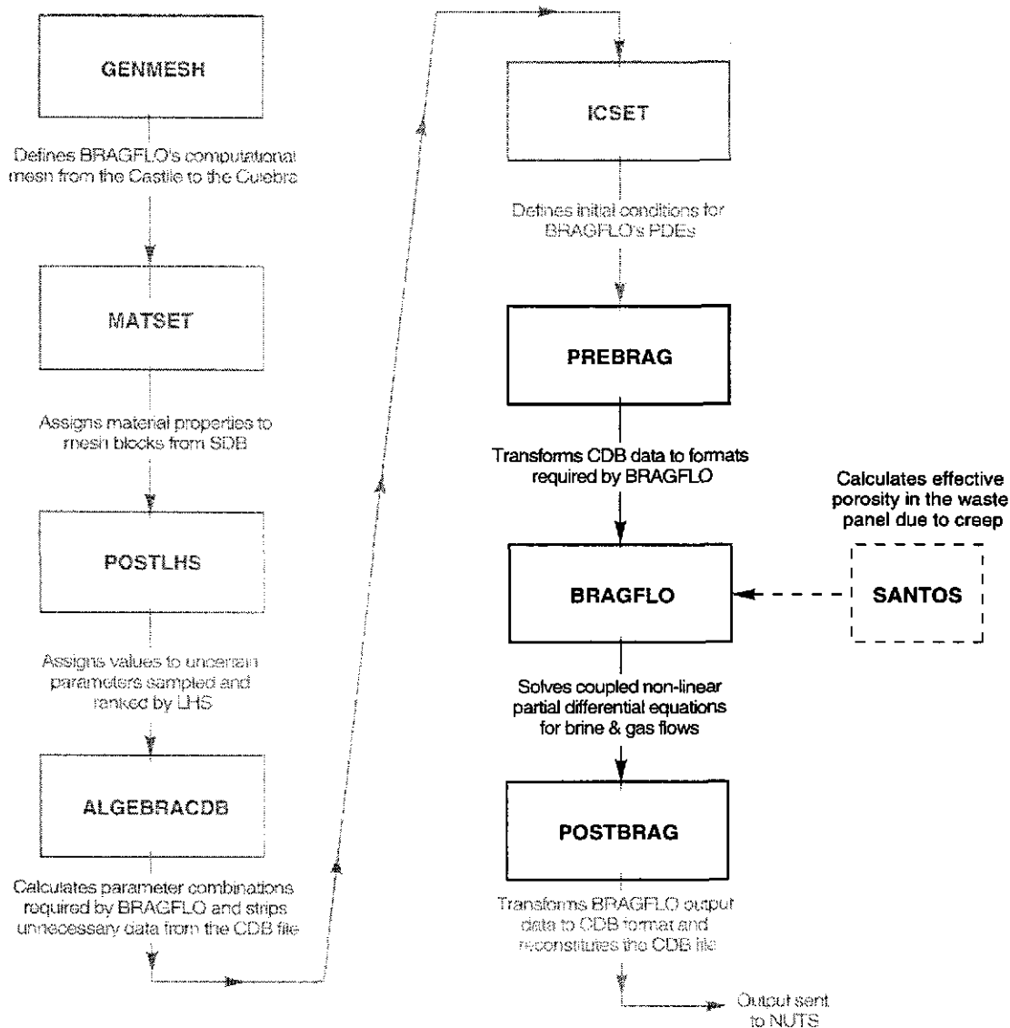
Figure 29. Sample computational flow diagram for BRAGFLO, highlighting flow to and from BRAGFLO.
