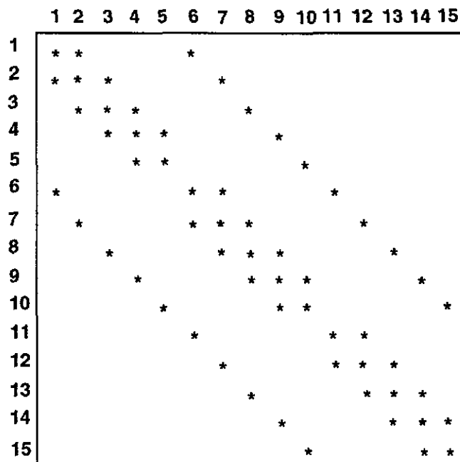
Figure 12. Jacobian matrix.
