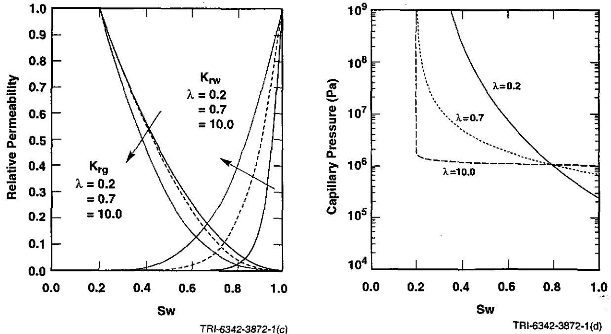
Figure 24. Relative Permeabilities for Brooks-Corey Model effect of pore size distribution parameter (left plot) and Capillary Pressure for Brooks-Corey Model effect of pore size distribution parameter (right plot).
