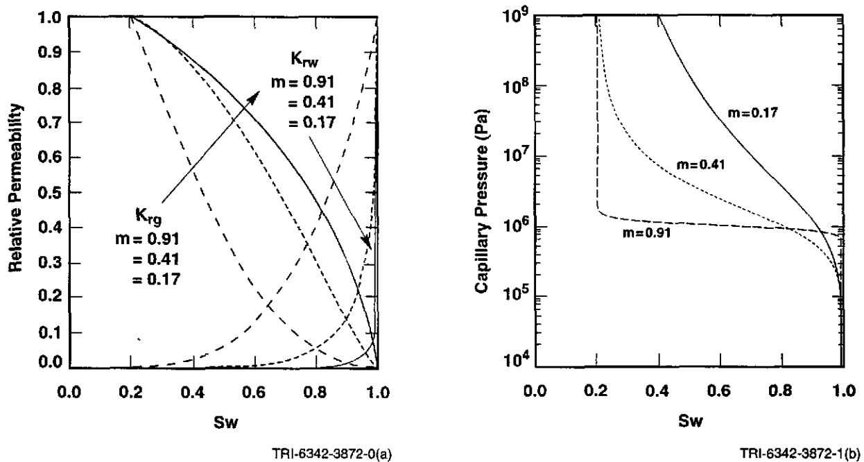
Figure 23. Relative Permeabilities for van Genuchten-Parker Model, effect of parameter m (left plot) and Capillary Pressure for van Genuchten-Parker Model, effect of parameter m (right plot).
