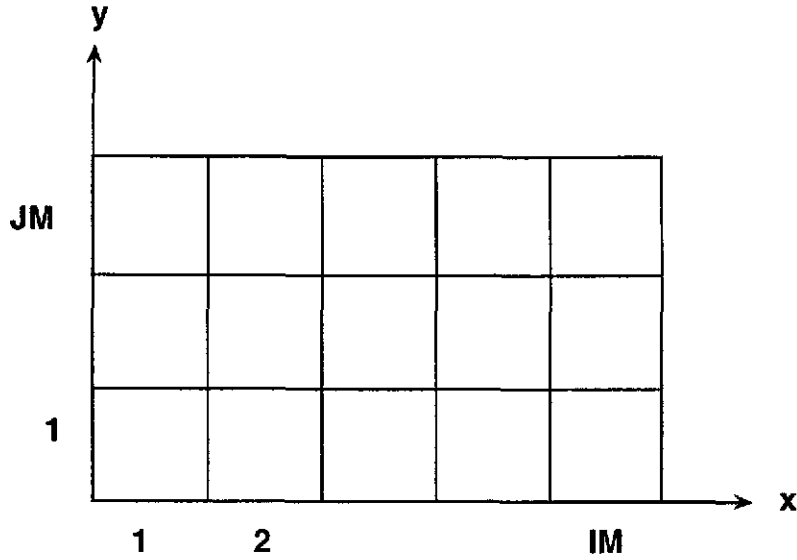
Figure 9. 2-dimensional grid.
