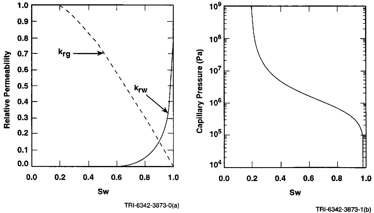
Figure 17. Relative Permeabilities for van Genuchten-Parker Model (left plot) and Capillary Pressure for van Genuchten-Parker Model (right plot).
